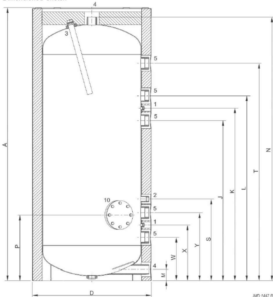
Dimensioned Sketch
